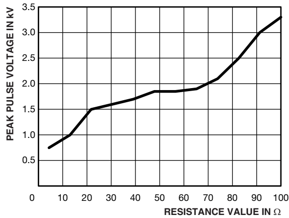
PEAK VOLTAGE LIMIT FOR AC01-CS (1.2 / 50 \mu s; 10 pulses at 30 s interval)
