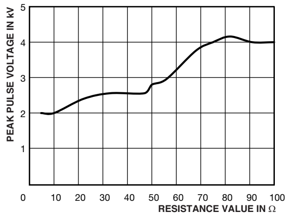
PEAK PULSE VOLTAGE LIMIT FOR AC03-CS (1.2 / 50 \mu s; 10 pulses at 30 s interval)
