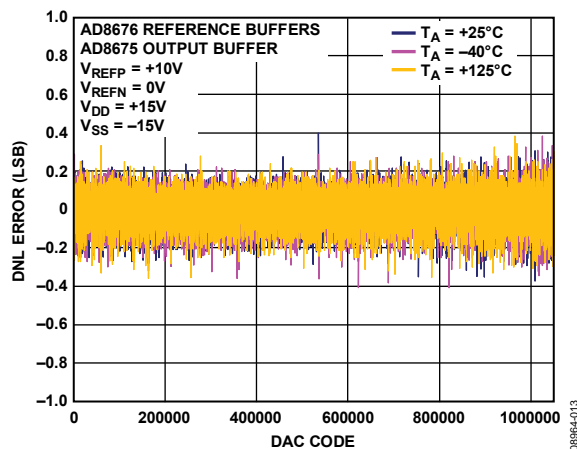
Figure 13. Differential Nonlinearity Error vs. DAC Code, \pm 10 V Span, X2 Gain Mode
