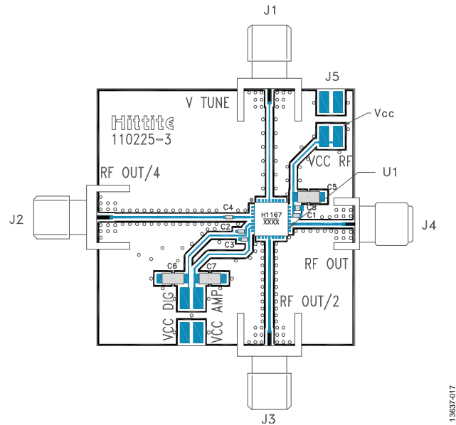
Figure 17. Evaluation PCB
