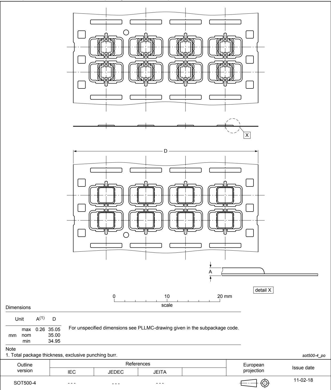
Figure 7. Package outline SOT500-4
