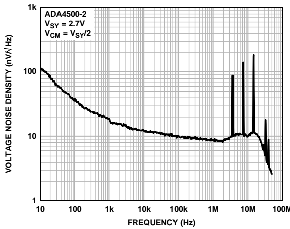
Figure 50. Voltage Noise Density vs. Frequency, V_{SV} = 2.7\text{V} (10 Hz to 100 MHz)
