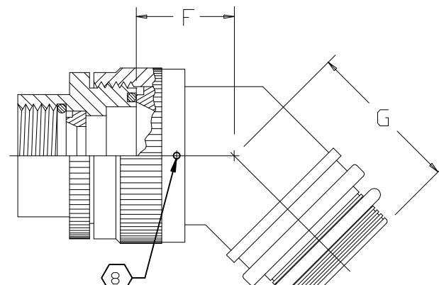
45° ADAPTER-TYPE II
