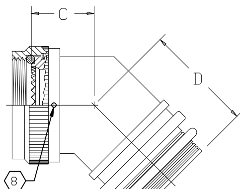
45° ADAPTER-TYPE I
