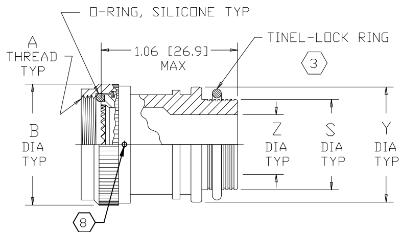
STRAIGHT ADAPTER-TYPE I
