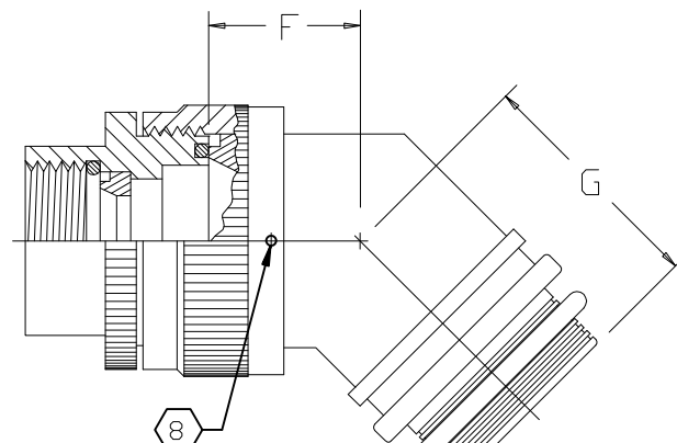
45° ADAPTER-TYPE II
