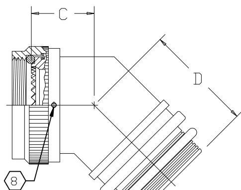
45° ADAPTER-TYPE I
