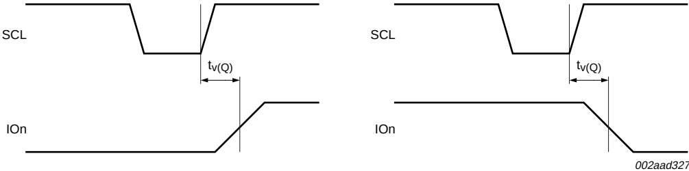
Fig 22. t_{v(Q)} timing
