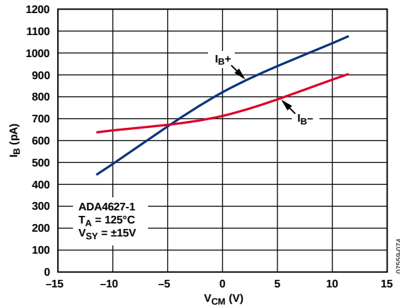
Figure 22. Input Bias Current vs. V_{CM} at 125°C
