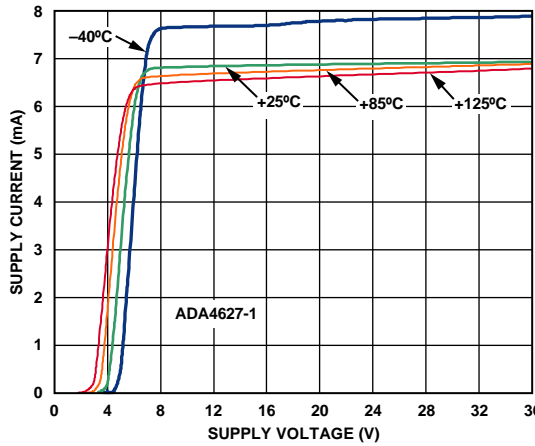
Figure 11. Supply Current vs. Supply Voltage and Temperature
