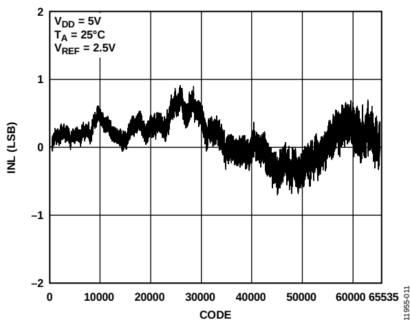
Figure 11. AD5683R/AD5683 INL
