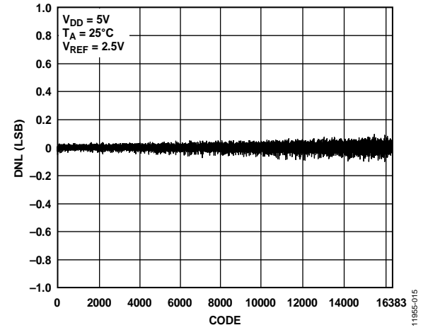
Figure 15. AD5682R DNL
