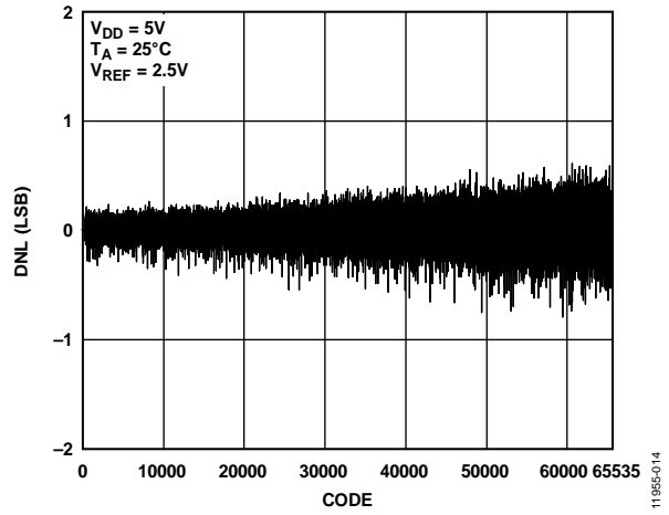
Figure 14. AD5683R/AD5683 DNL
