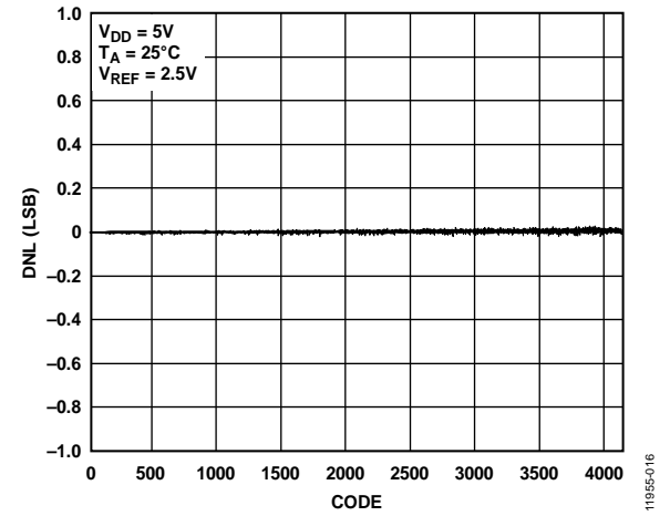
Figure 16. AD5681R DNL
