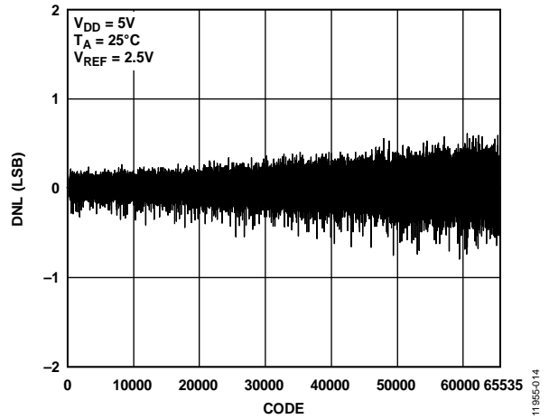
Figure 14. AD5683R/AD5683 DNL
