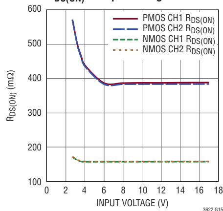
R_{DS(ON)} vs Input Voltage
