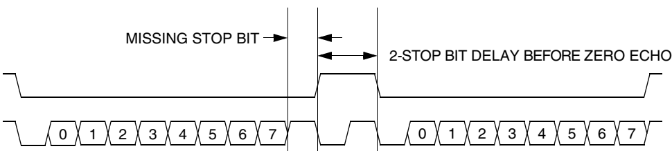
Figure 10-4. Break Transaction
