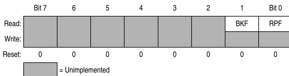
Figure 16-14. SCI Status Register 2 (SCS2)
