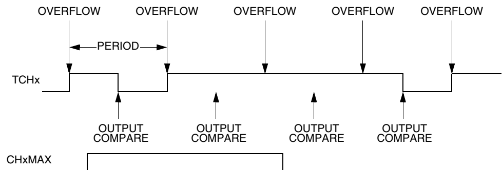
Figure 11-11. CHxMAX Latency
