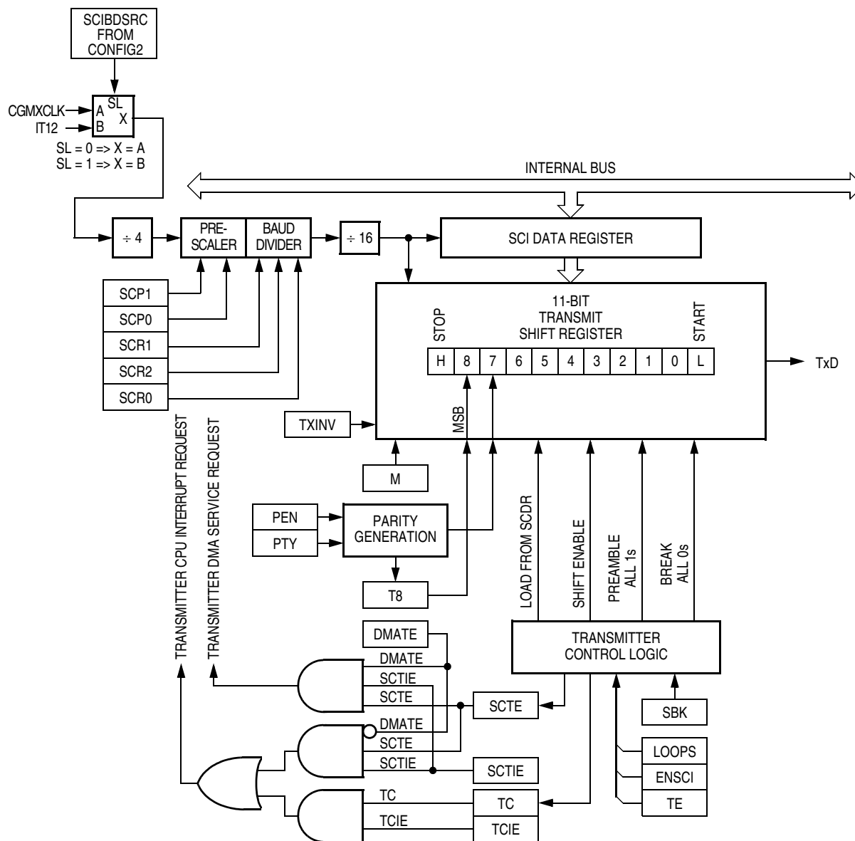
Figure 16-4. SCI Transmitter
