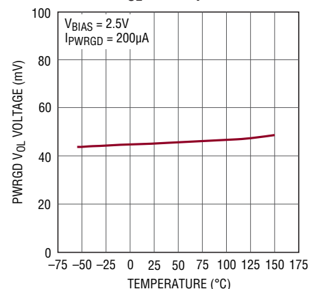
PWRGD V_{OL} vs Temperature
