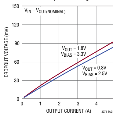
Dropout Voltage
