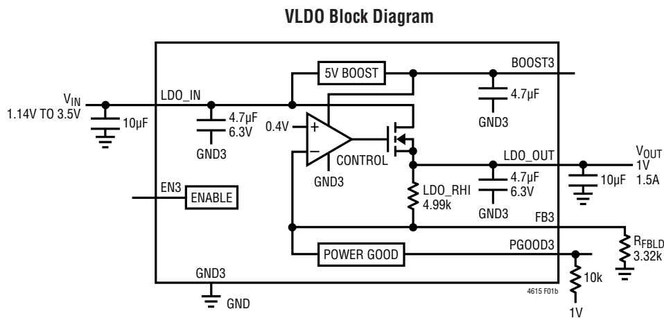
Figure 1. Simplified LTM4615 Block Diagram of Each Switching Regulator Channel and the VLDO
