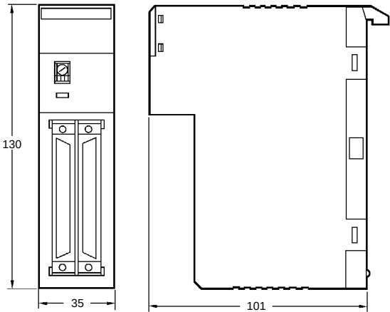
Group-2 High-density I/O Units (C and D Types)
