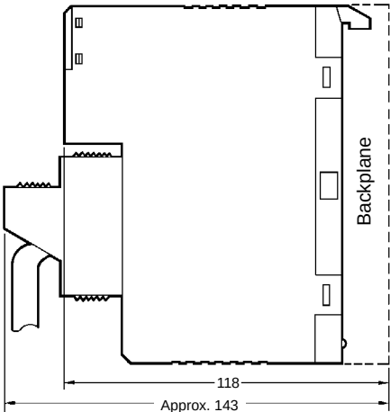
Dimensions with Unit Mounted
