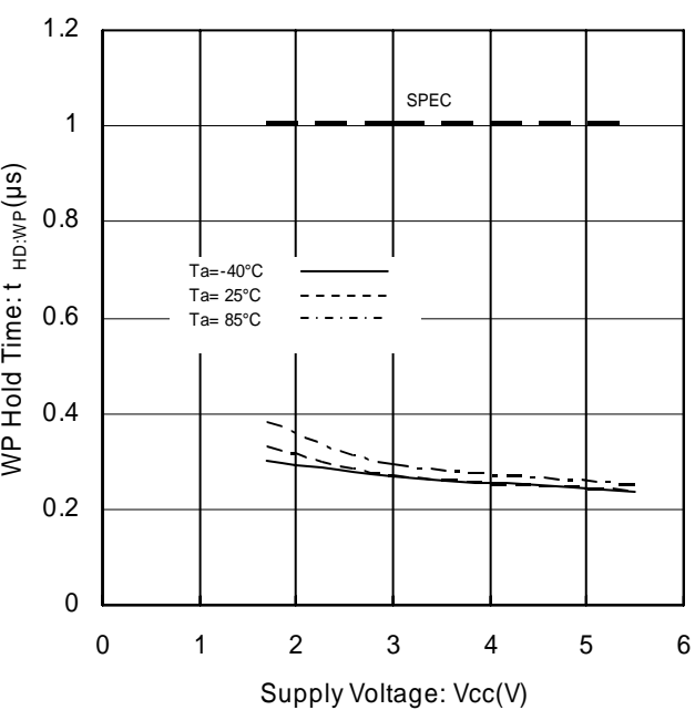
Figure 31. WP Hold Time vs Supply Voltage
