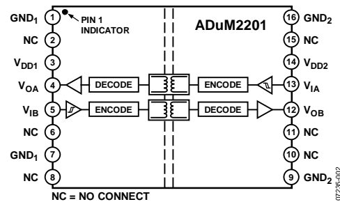
Figure 2. ADuM2201
