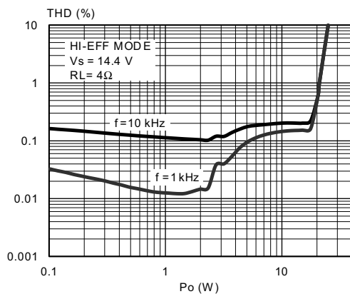
Figure 10. Distortion vs. output power (4 Ω, HI-EFF)
