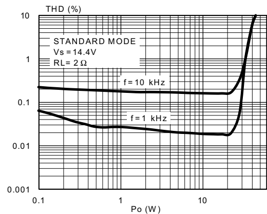
Figure 11. Distortion vs. output power (2 Ω, STD)
