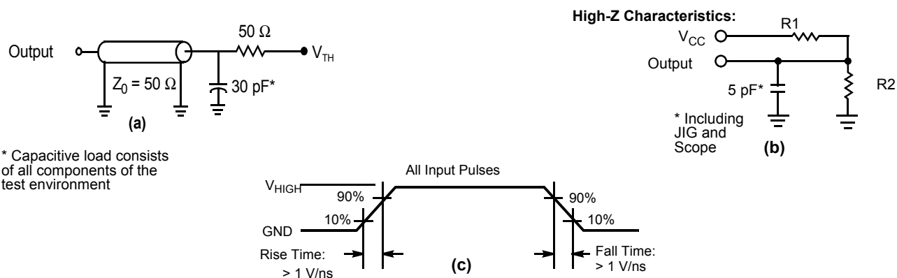
Figure 3. AC Test Loads and Waveforms [9]
