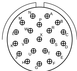
Front face of pin inserts illustrated
