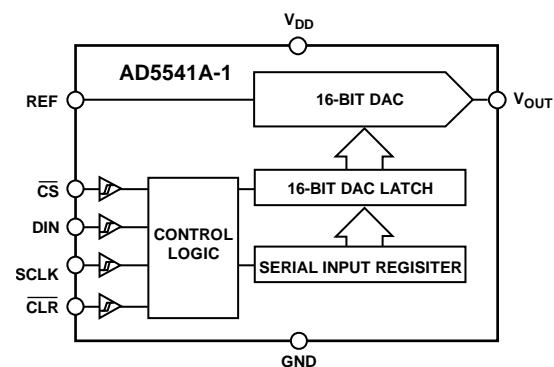
Figure 2. AD5541A-1
