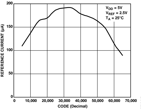
Figure 18. Reference Current vs. Code
