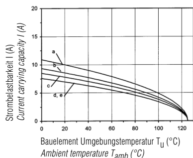
Derating Kurven / Derating curves
