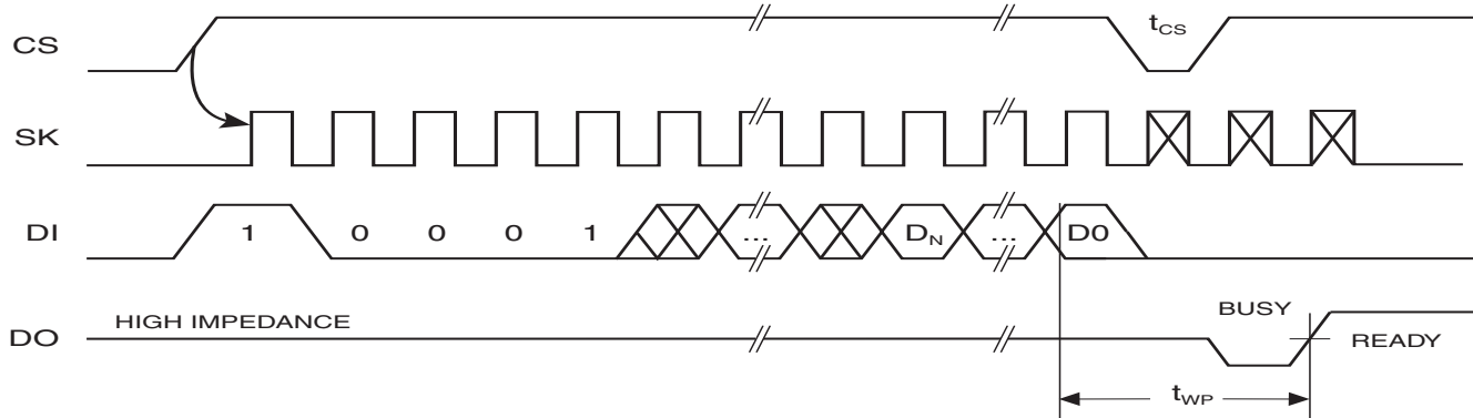
Figure 4-6. WRAL Timing (1),(2)
