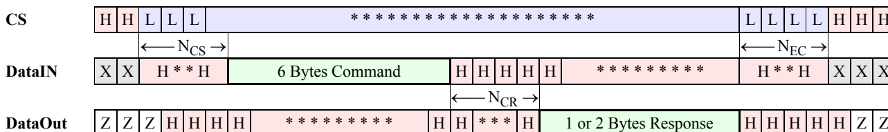
Figure 7-15 : SPI Command/Response Transaction, Card Is Ready
