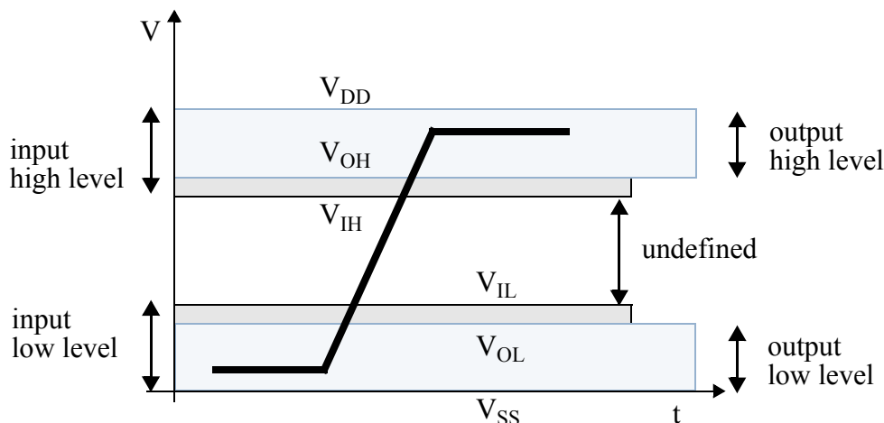
Figure 5-4 : Bus Signal Levels
