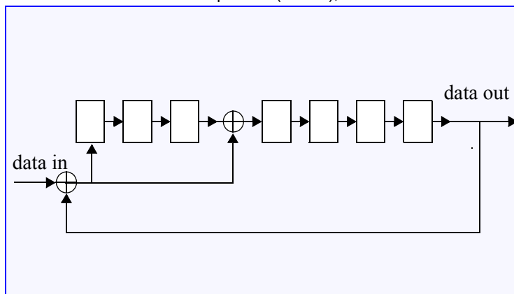
Figure 6-3 : CRC7 Generator/Checker
