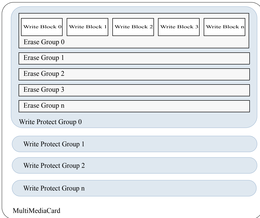
Figure 6-5 : Memory Array Partitioning
