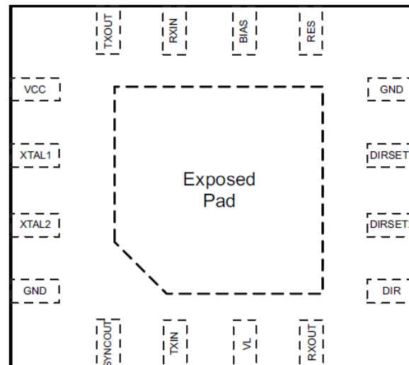
Figure 1. SN65HVD62 Pinout
