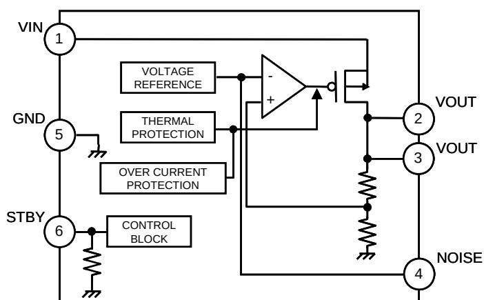
Figure 2. Block diagram
