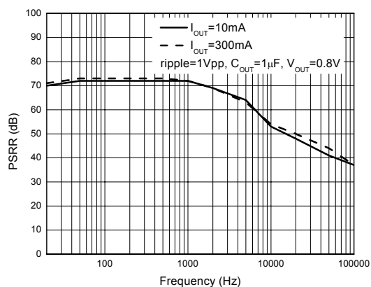
Figure 19. PSSR vs. Frequency
