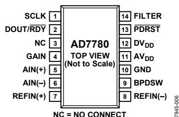
Figure 6. SOIC Pin Configuration
