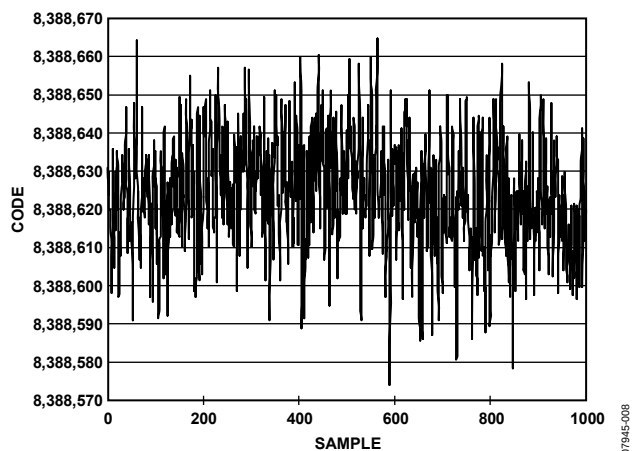
Figure 8. Noise ( V_{REF} = AV_{DD} , Update Rate = 16.7 Hz, Gain = 128)
