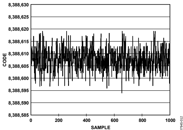
Figure 12. Noise ( V_{REF} = AV_{DD} , Update Rate = 16.7 Hz, Gain = 1)
