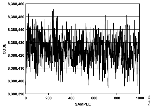
Figure 10. Noise ( V_{REF} = AV_{DD} , Update Rate = 10 Hz, Gain = 128)
