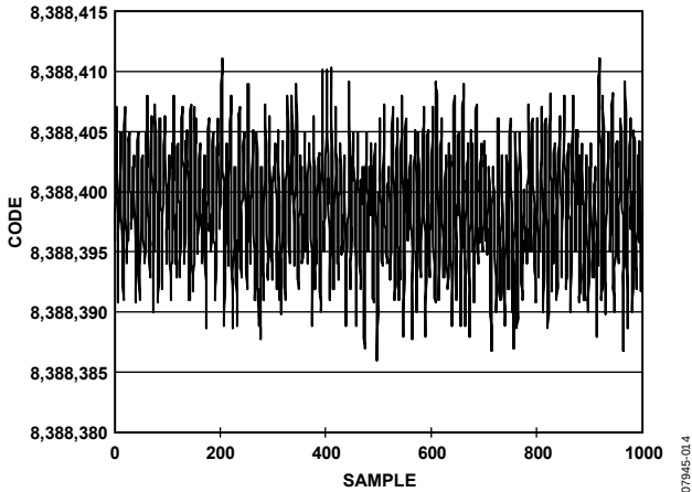
Figure 14. Noise ( V_{REF} = AV_{DD} , Update Rate = 10 Hz, Gain = 1)
