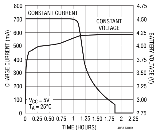
Complete Charge Cycle (900mAh Battery)
