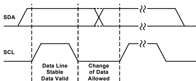
Figure 27. Data Validity
