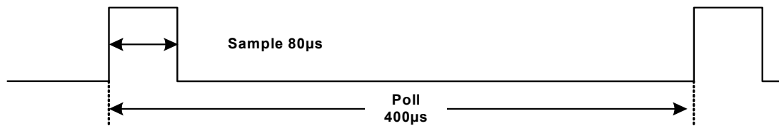
Figure 36. ADC Sample and Polling Time
