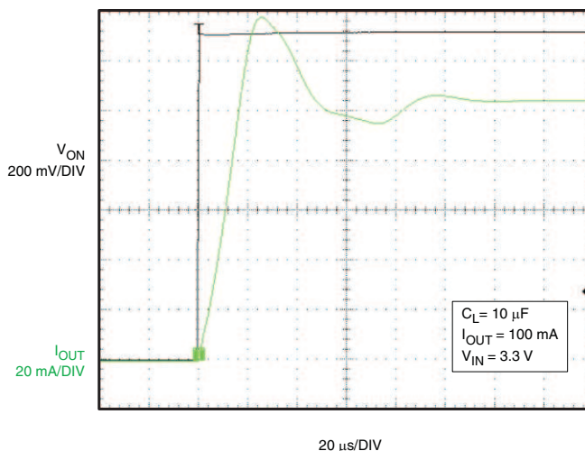
Figure 19. t_{ON} Response
