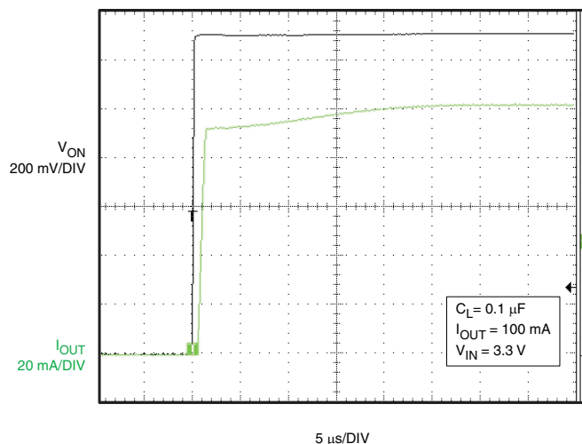
Figure 18. t_{ON} Response
