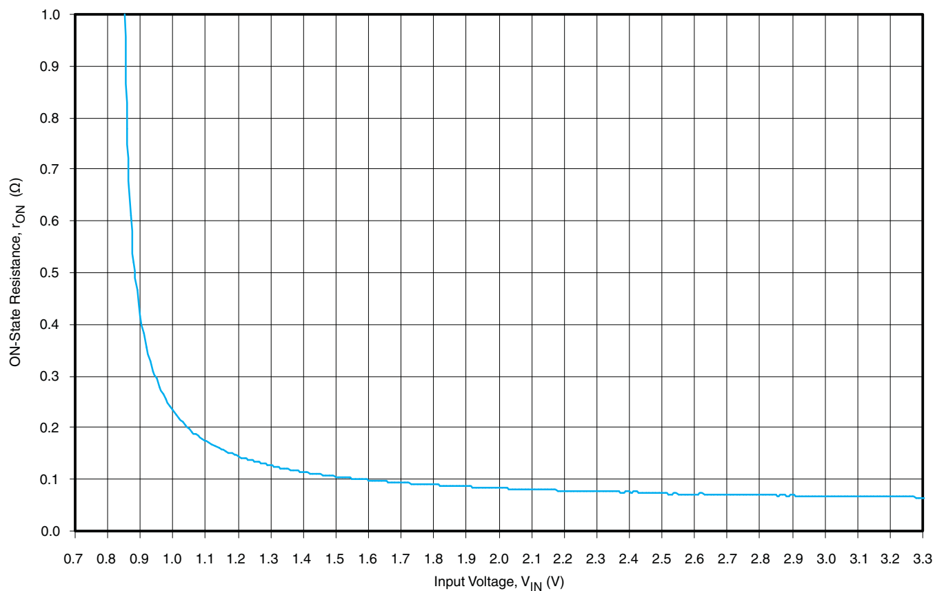
Figure 2. r_{ON} vs V_{IN}
