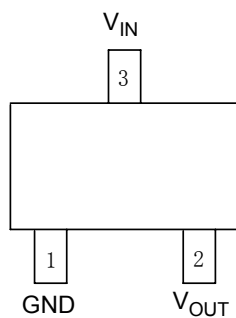
Figure 2. Pin Configuration of AP2120 (Top View)
