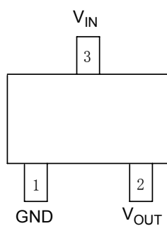
Figure 2. Pin Configuration of AP2120 (Top View)
