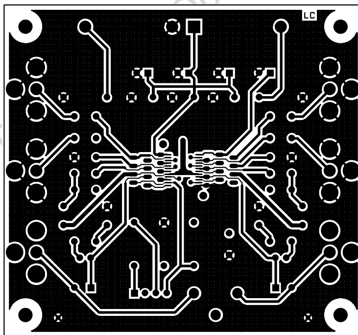
Figure 10. TDA7469 P.C. Board Layout (Top view)
