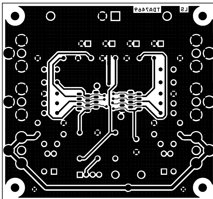
Figure 11. TDA7469 P. C. Board (Backside view)
