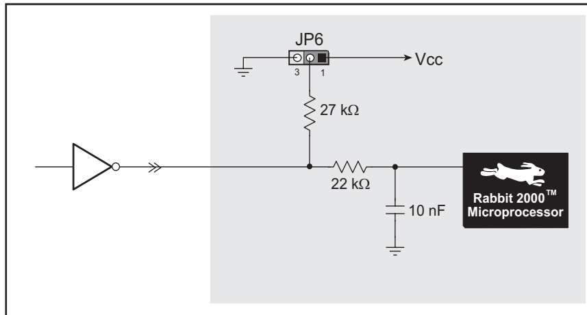
Figure 7(c). Example of Logic Gate Driving BL2000 Digital Input
