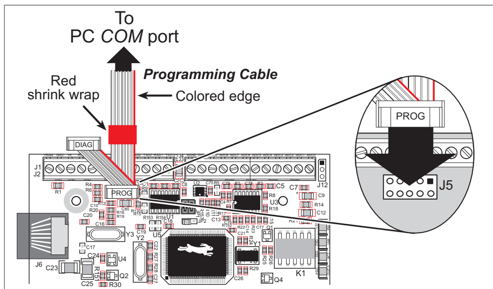
NOTE: Never disconnect the programming cable by pulling on the ribbon cable. Carefully pull on the connector to remove it from the header. NOTE: Some PCs now come equipped only with a USB port. It may be possible to use an RS-232/USB converter (Part No. 20-151-0178) with the programming cable supplied with the Tool Kit. Note that not all RS-232/USB converters work with Dynamic C.
