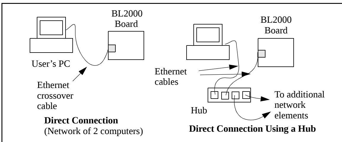
Figure 21. Ethernet Connections
