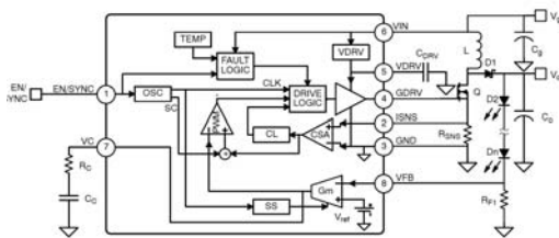
Figure 4. Simplified Typical Single Channel Converter
