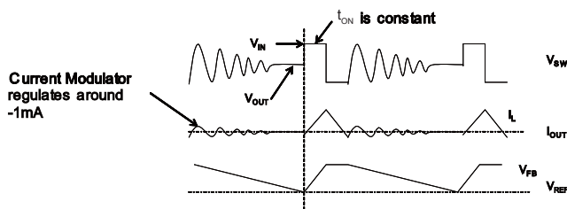
Figure 2: Light-Load Operation
