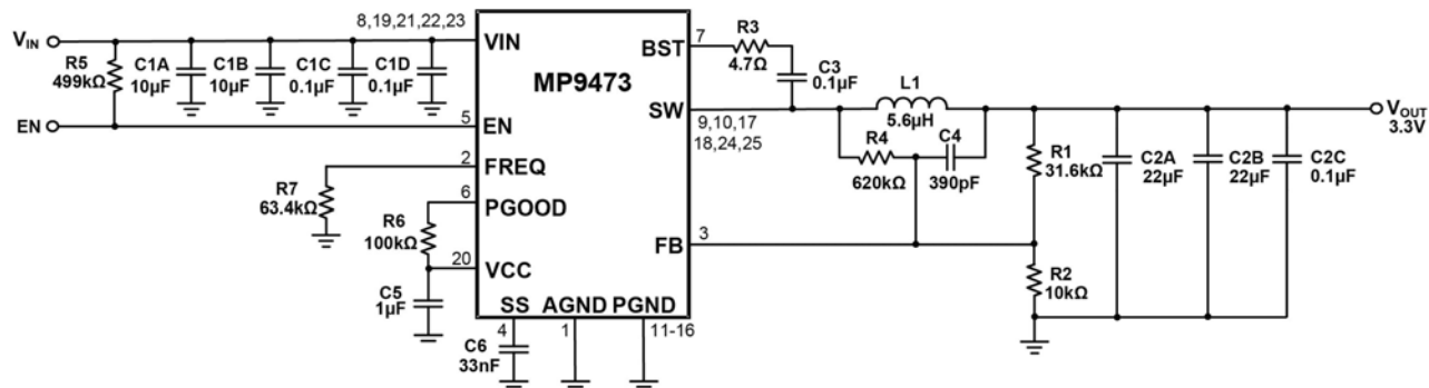
Figure 10: Typical Application Circuit, 3.3V-Output
