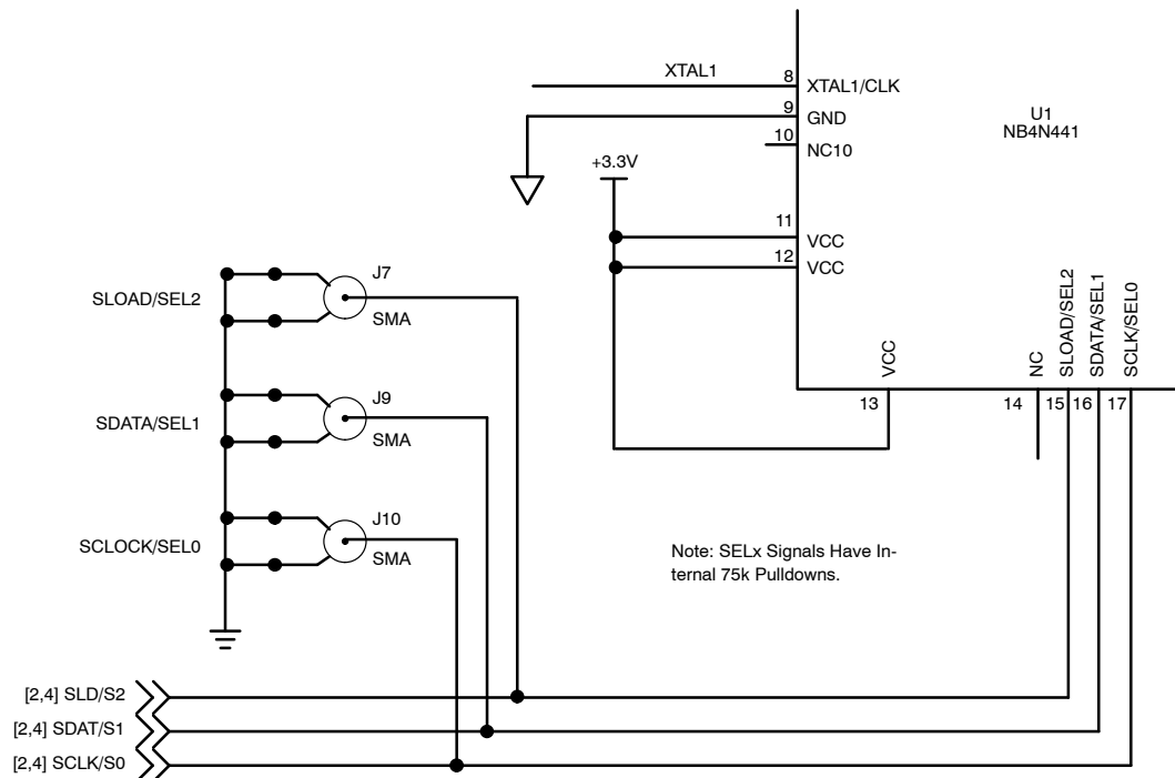
Figure 5. SDI Inputs
