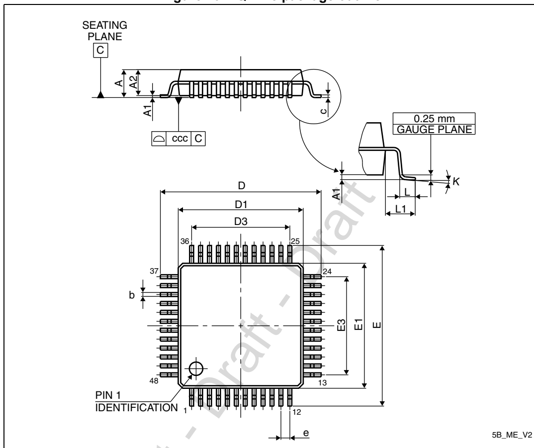
Figure 40. LQFP48 package outline
