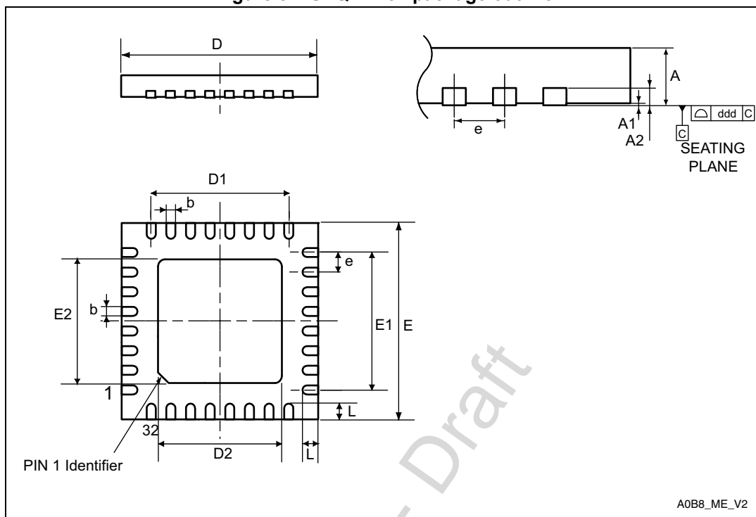
Figure 52. UFQFPN32 package outline
