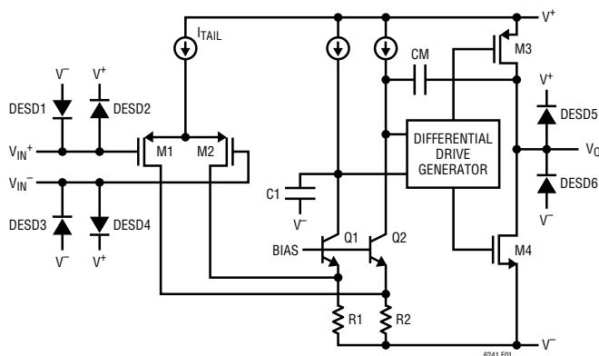
Figure 1. Simplified Schematic
