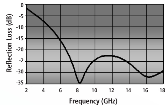
Typical electrical performance
