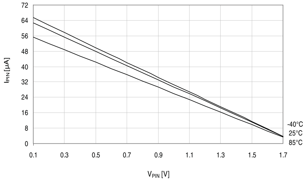
Figure 34-101. I/O pin pull-up resistor current vs. input voltage. V_{CC} = 3.0V .
