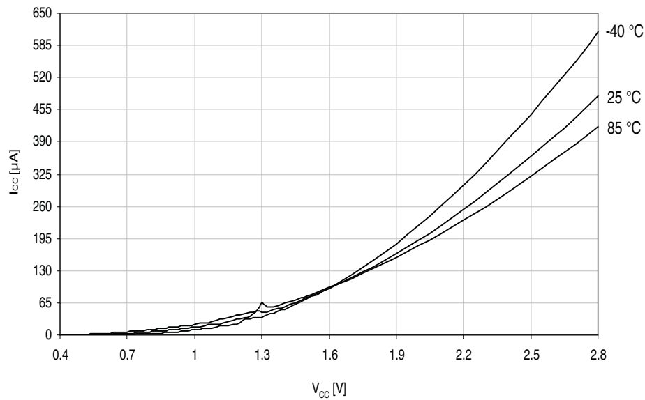
Figure 34-64. Power-on reset current consumption vs. V_{CC} . BOD level = 3.0V, enabled in sampled mode.
