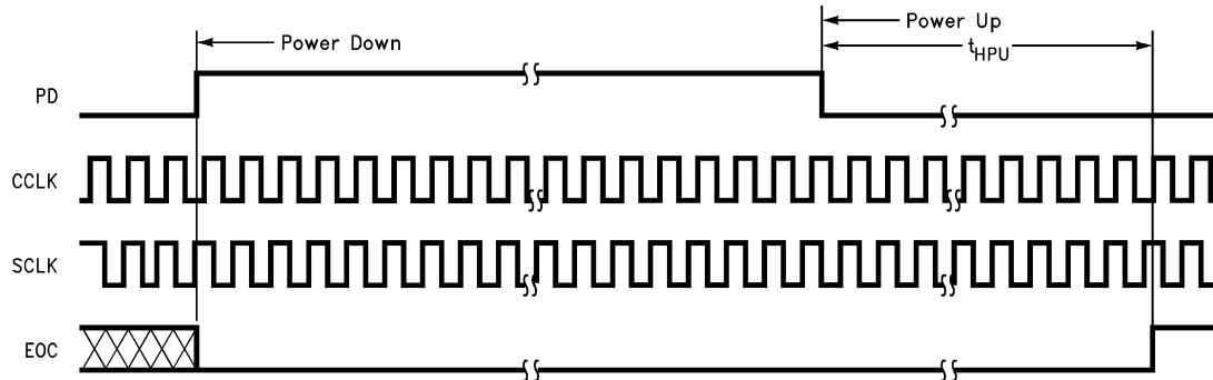
ADC12L038 Hardware Power Up/Down
