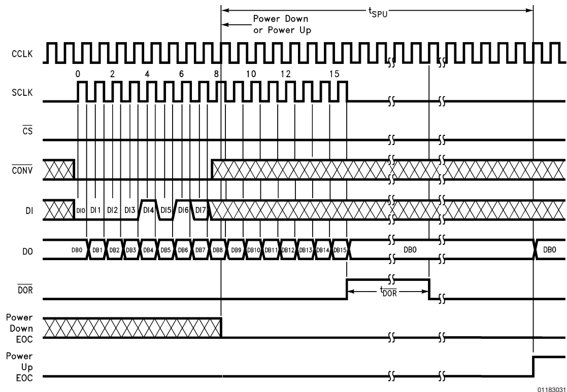
ADC12L038 Hardware Power Up/Down
