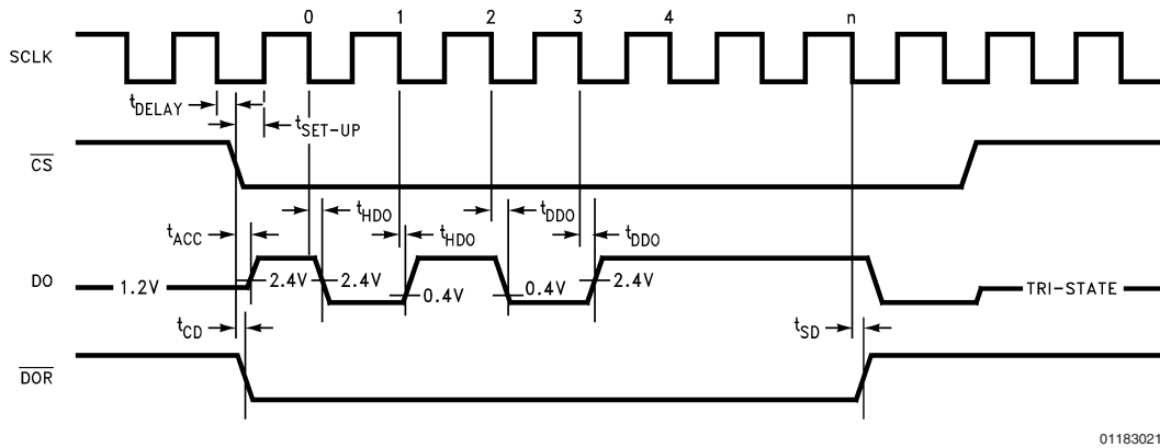
DO Data Output Timing with \overline{CS} Continuously Low
