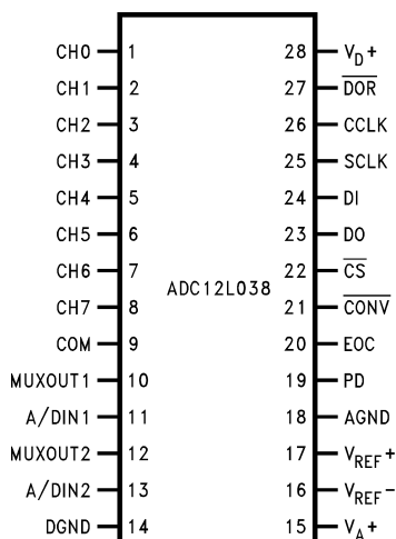
28-Pin Wide Body SO Package
