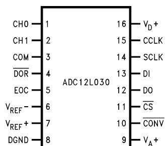
16-Pin Wide Body SO Package
