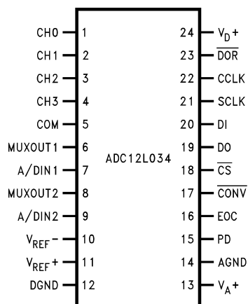
24-Pin Wide Body SO Package
