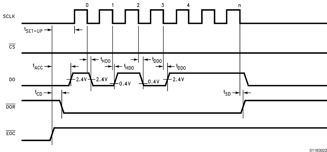
DO Data Output Timing with \overline{CS} Continuously Low
