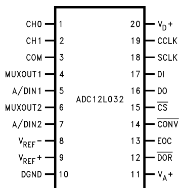
20-Pin Wide Body SO Package
