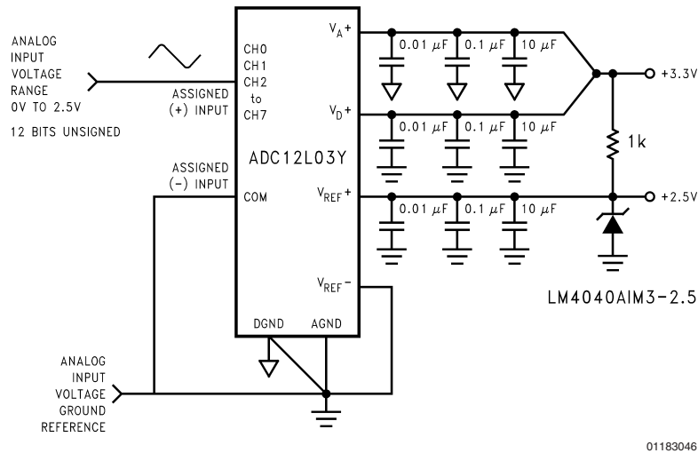
FIGURE 11. Single-Ended Biasing
