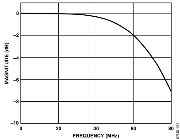
Figure 91. Band-Pass Filter Pass-Band Detail, f DAC = 2.4 GHz
