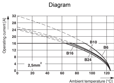
The figure shows the derating diagram of various series B contact inserts (B6 to B24), conductor cross section 2.5 mm 2
